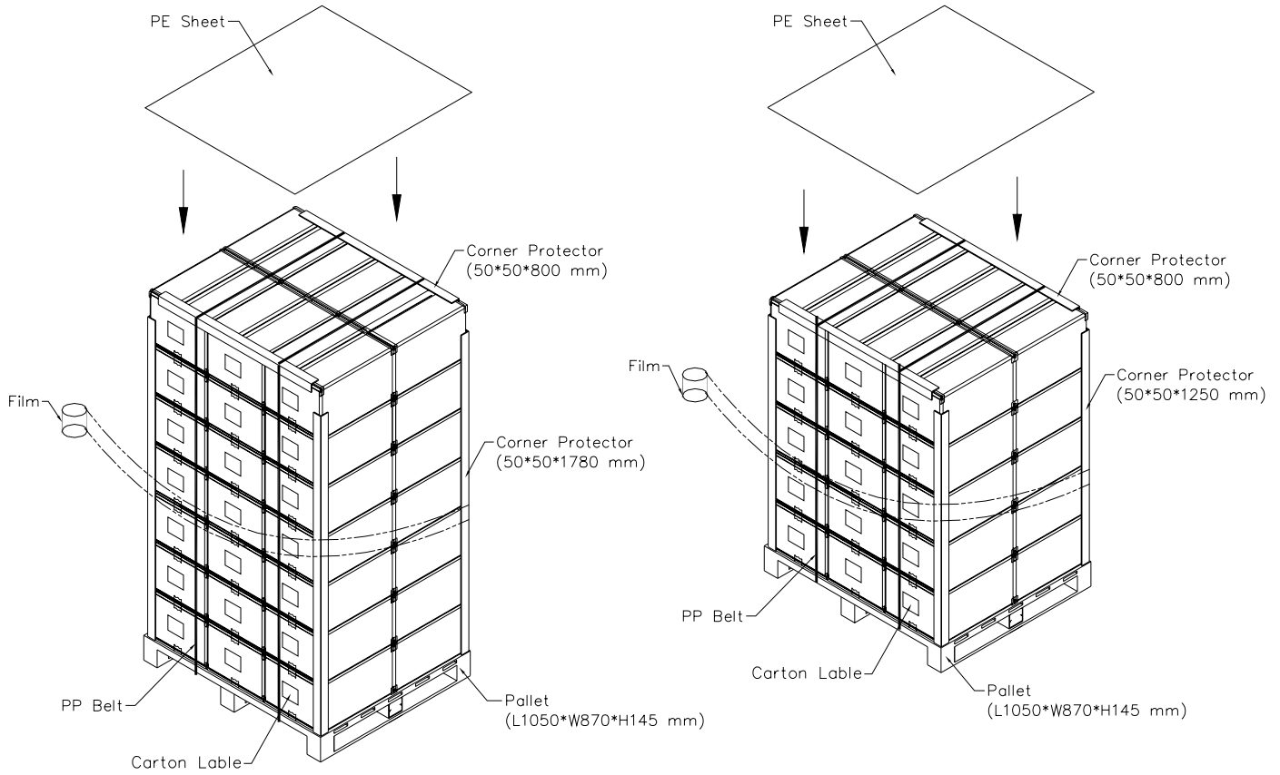
Figure. 10-2 Packing method
